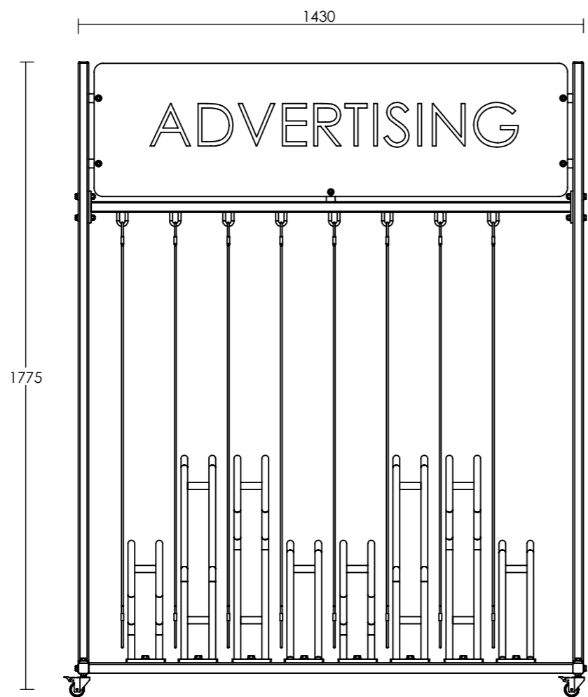
Front View
