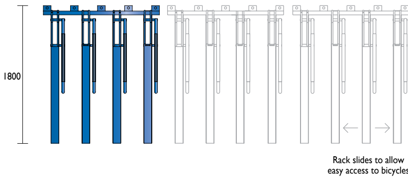
Front View 1500
