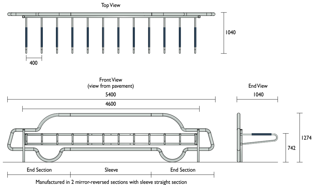
Standard Parking Spaces 5400 x 2400
