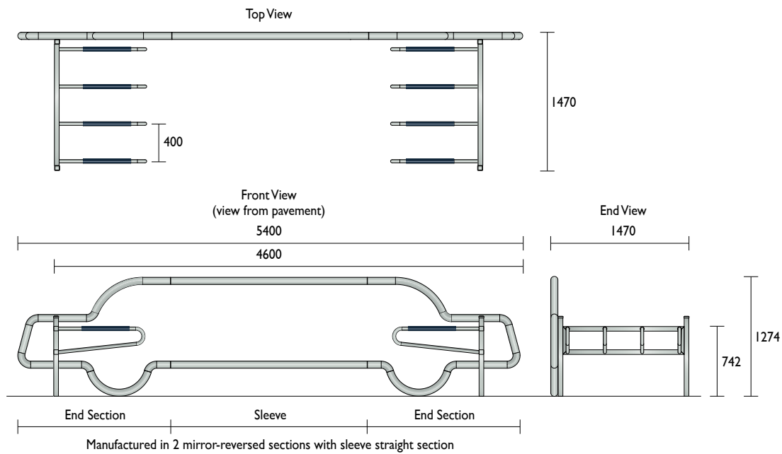
Standard Parking Spaces 5400 x 2400
