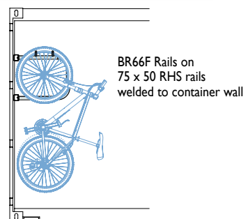
End Sectional View 1050 Nominal
